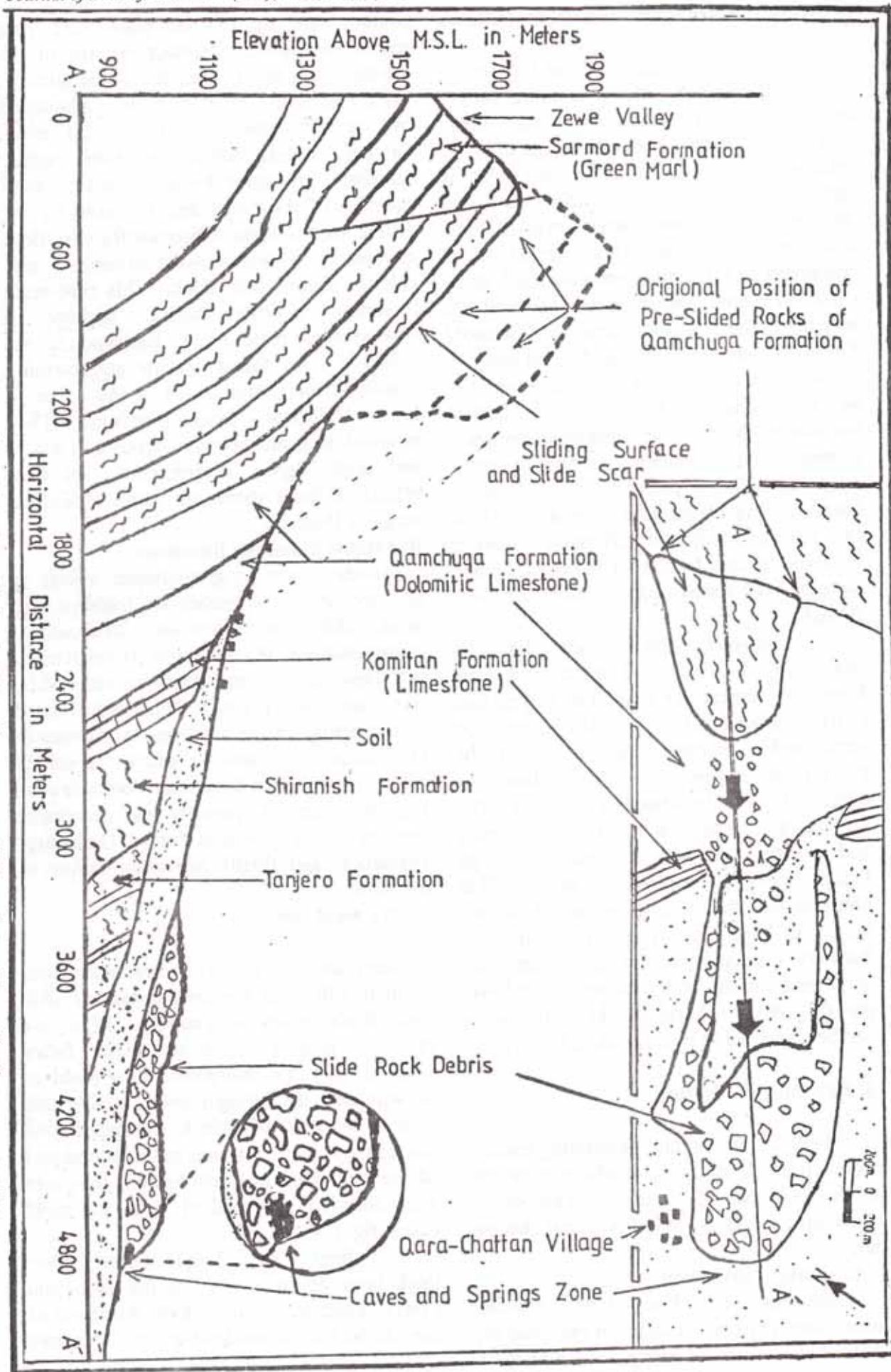
Fig.(3) Geological cross-section of southwestern limb of Pira-Magroon anticline along Qara-Chattan rockslide.
